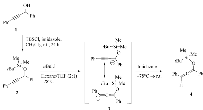
Scheme 2. Synthesis of tert -butyldimethylsilyl ether 4 .
