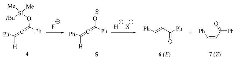
Scheme 3. Generation and kinetic protonation of 1,3-diphenylallenolate 5 .
