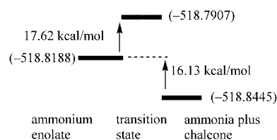
Scheme 5. B3LYP computations (energies in parentheses are in Hartrees).
